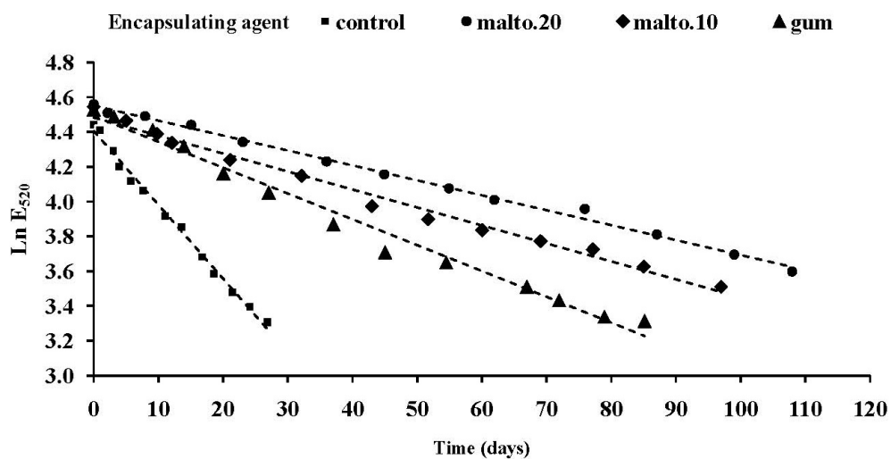
Fig. 5: First-order degradation plots for roselle anthocyanins encapsulated in different matrices during storage at aw 0.64 and temperature 35°C
