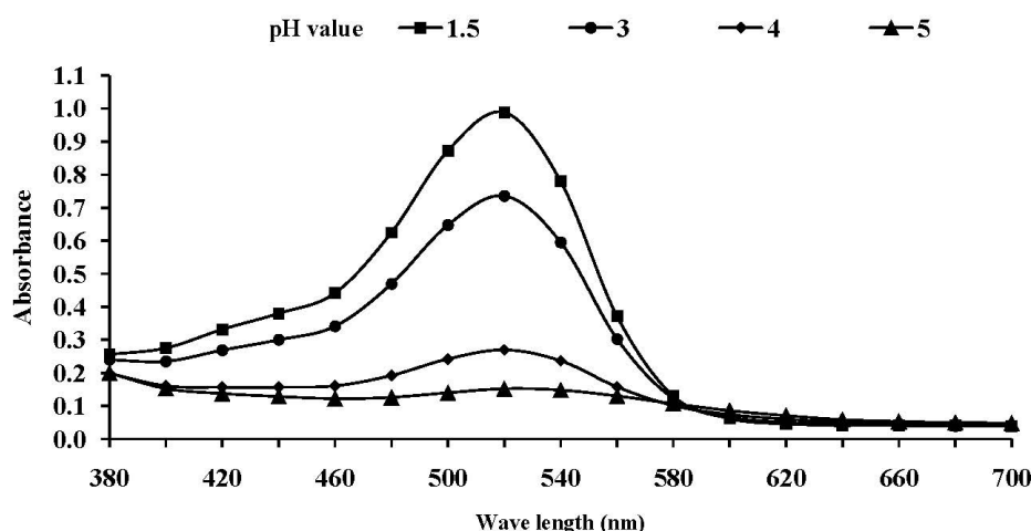
Fig. 1: Absorption spectrum of roselle anthocyanins
