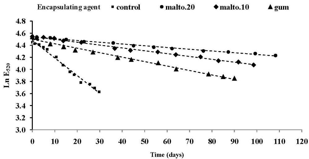
Fig. 4: First-order degradation plots for roselle anthocyanins encapsulated in different matrices during storage at aw 0.53 and temperature 35°C
