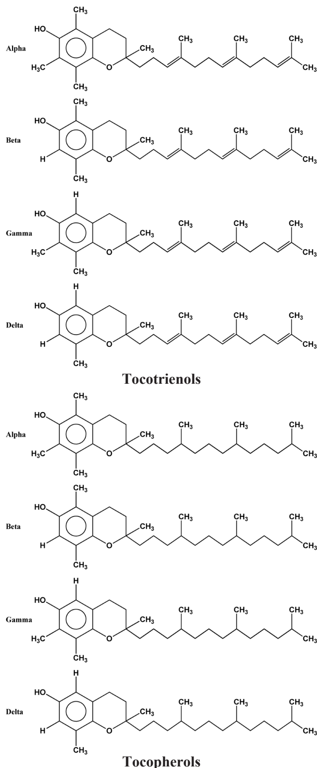
Fig. 3: Chemical formulas of tocopherols and tocotrienols
